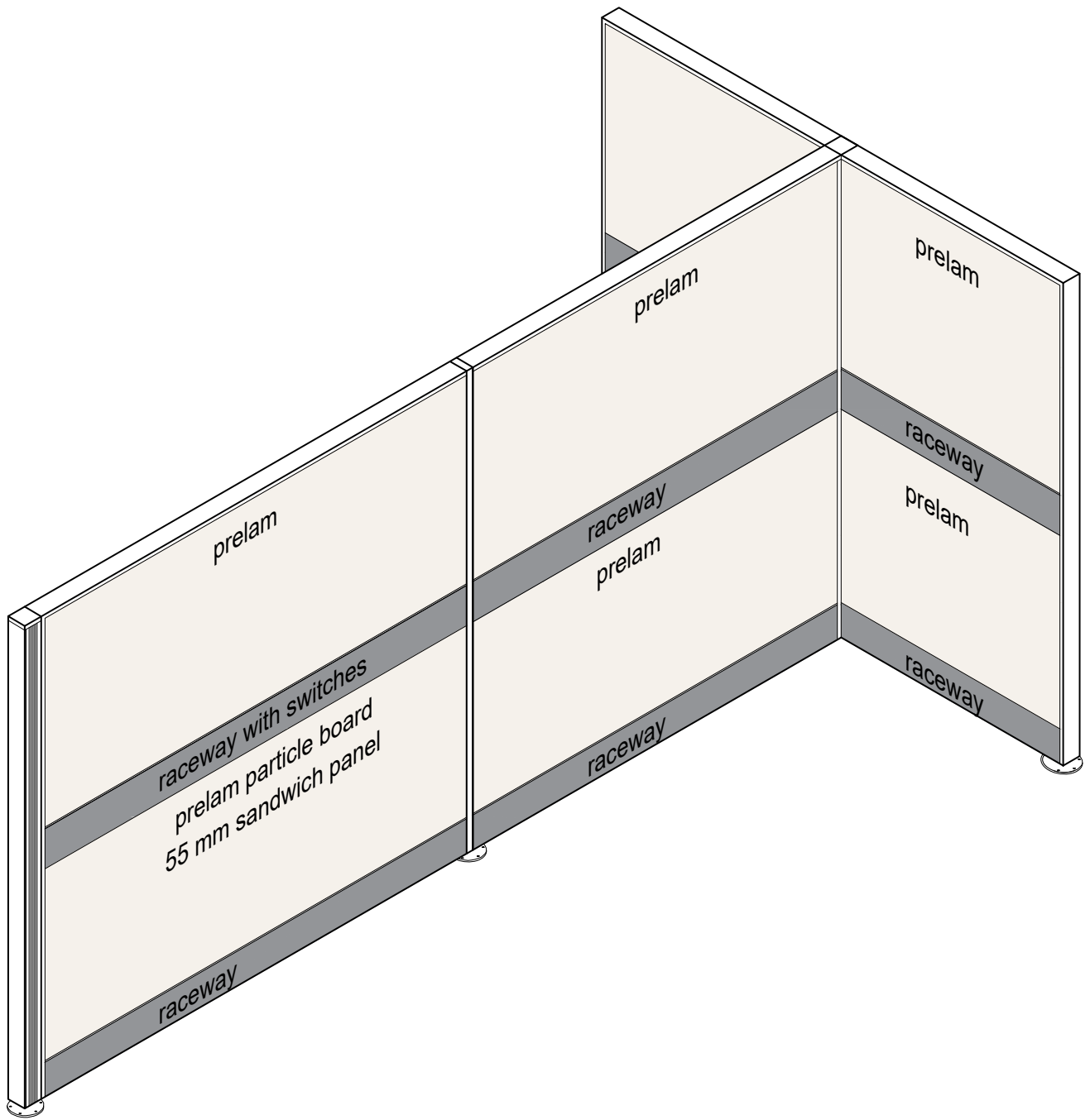
Isometric View
